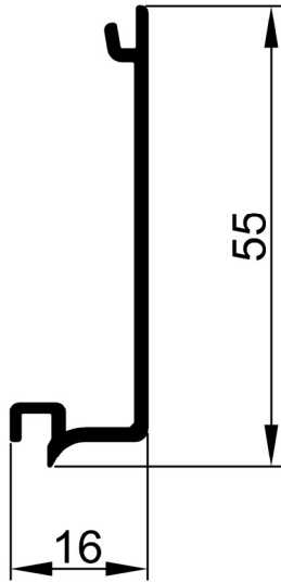
45 SL 50 Kenet Profili/Sash Profile Ağırlık :0,32 kg/m (Weight)
