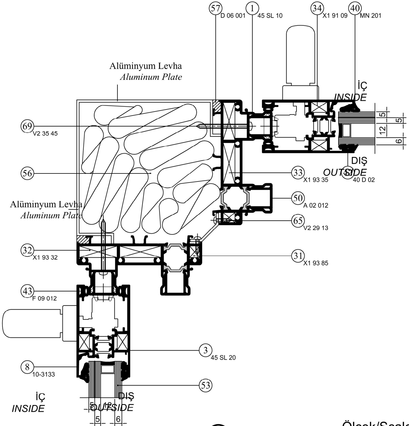
DETAIL ① DETAYI
